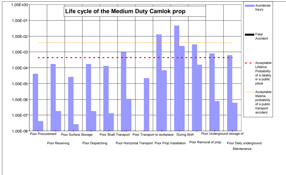
Figure 2: Risk profile of the Medium-duty Camlok Prop
